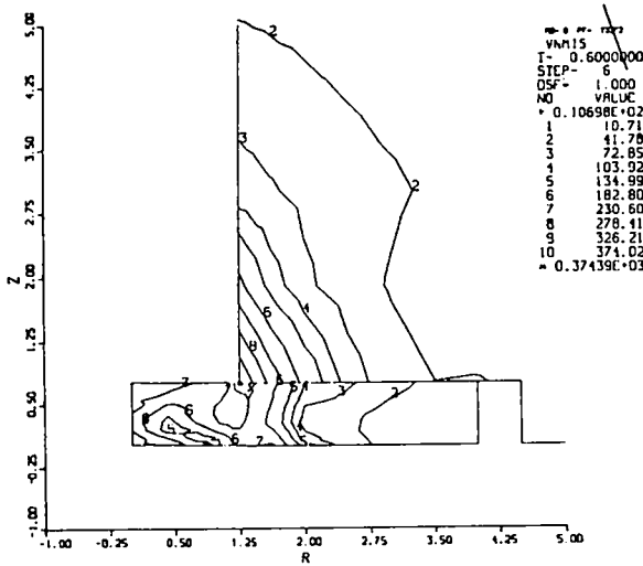
Fig. 25 Von Mises stress contours for a 0.75-mm-thick plate and a 2.5-mm-diam barrel. The pressure is 150 MPa.
