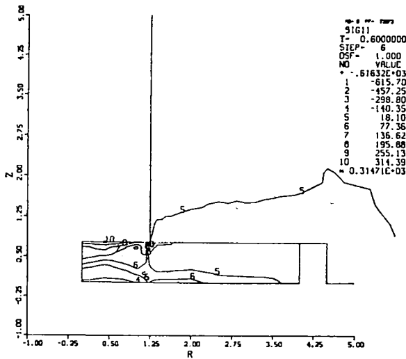
Fig. 29 First principal stress contours for a 0.75-mm-thick plate and a 2.5-mm-diam barrel. The pressure is 150 MPa.
